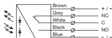
SPRR / SPPR / SPP / SPBS 29xx
