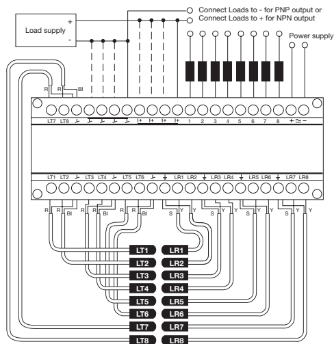
MPA 81 A/C 60x (Transistor Output)
