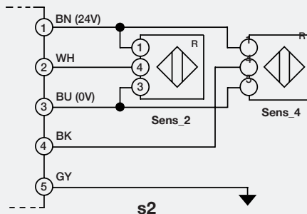
Receiver
