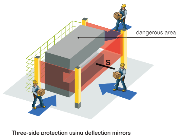
Three-side protection using deflection mirrors
