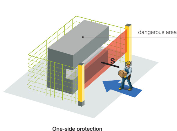
One-side protection
